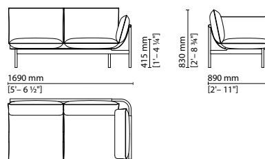
047010 — 2-seater sofa dx
