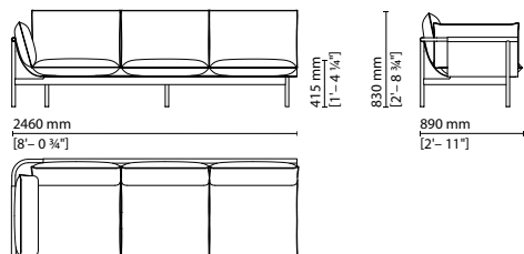
047007 — 3-seater sofa sx
