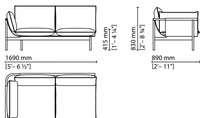
047009 — 2-seater sofa sx
